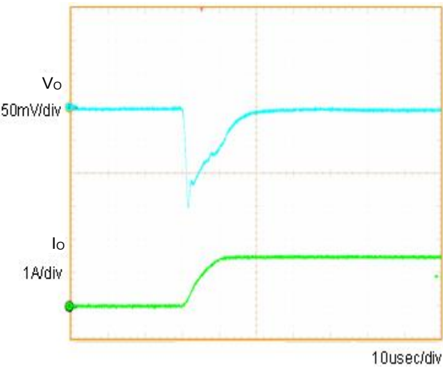
Fig.3 Transient Response (0→1.5A) Co=1µF
