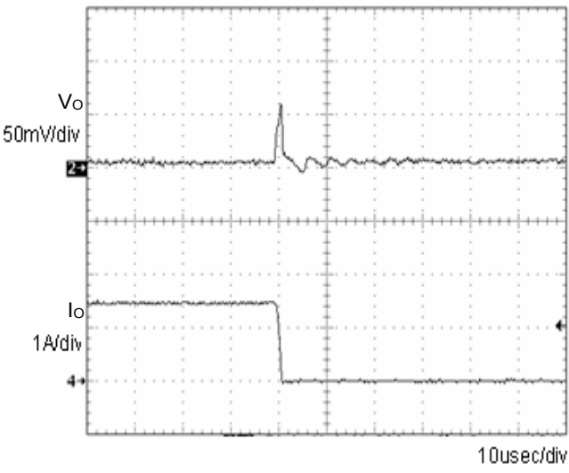
Fig.4 Transient Response (1.5→0A) Co=1µF
