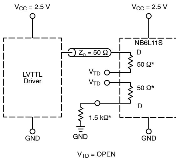
Figure 16. LVTTL Interface
