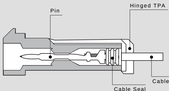
Male Connector
