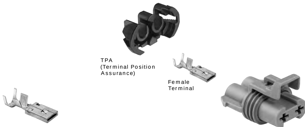
Female Connector
