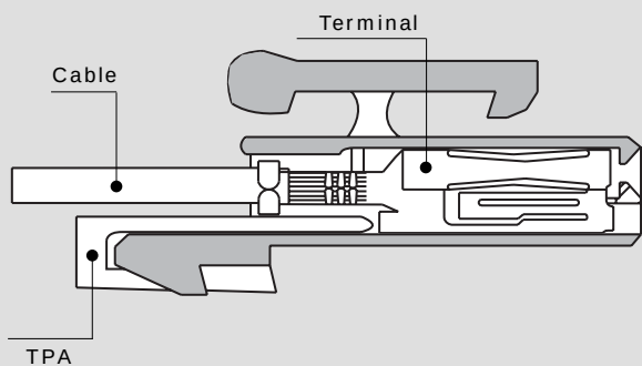
Female Connector
