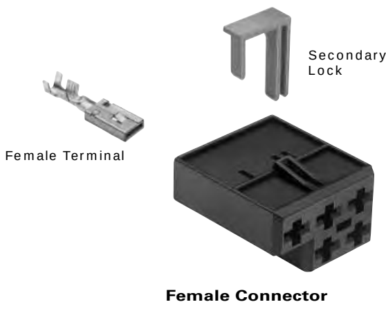
4.8 Female Connectors Unsealed
