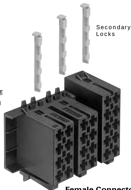
Female Connector Assembly
