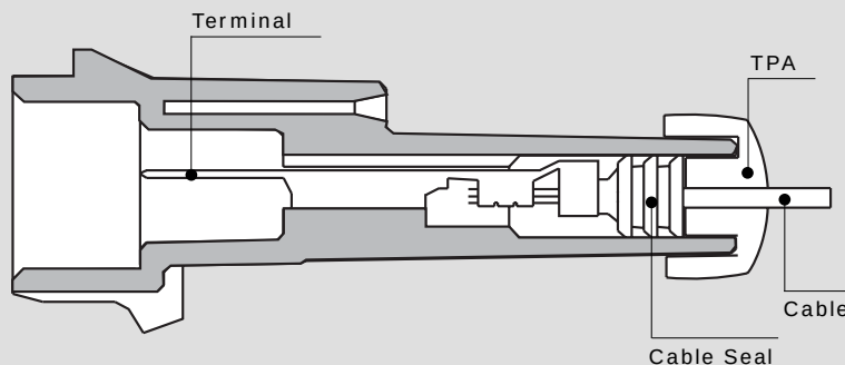
Male Connector
