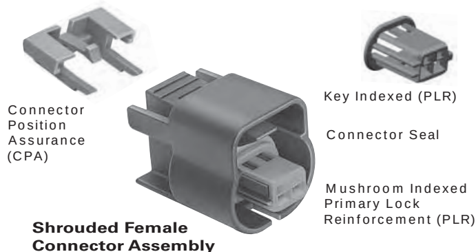
GT 150 Female Shrouded Connector Assemblies Sealed
