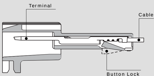
Male Connector
