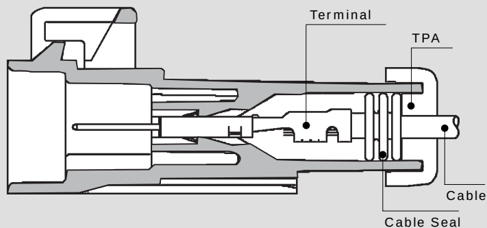
Male Connector
