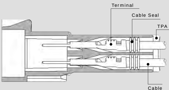
Male Connector
