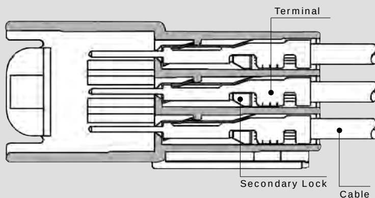
Male Connector
