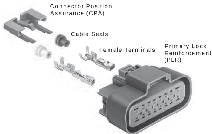
Female Connector Assembly
