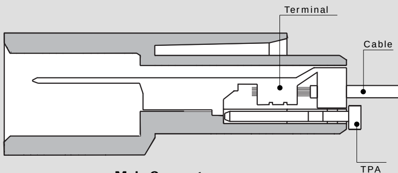
Male Connector
