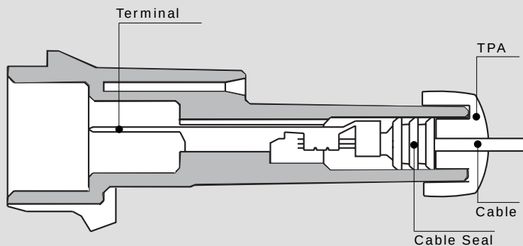
Male Connector
