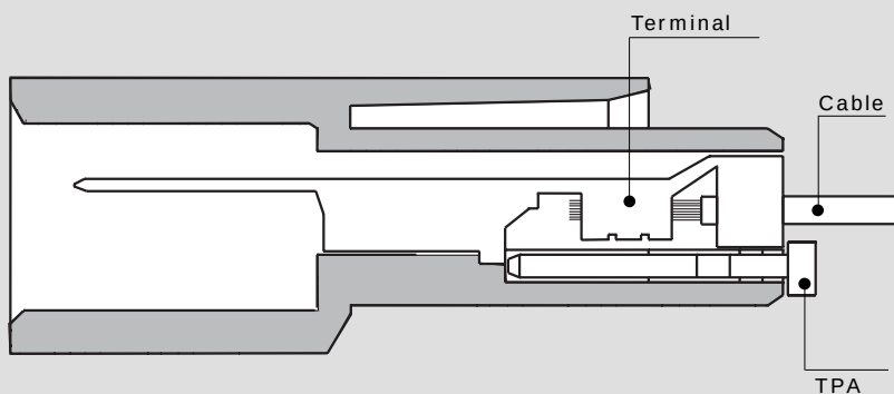
Male Connector
