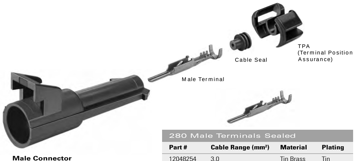
Male Connector
