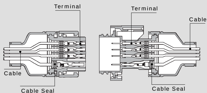
Male Connector
