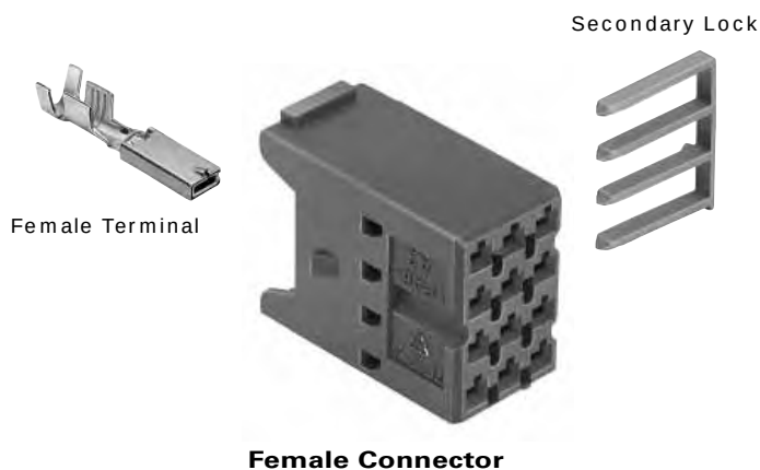
Female Connector
