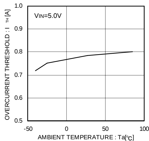
Figure 13. Over-current threshold
