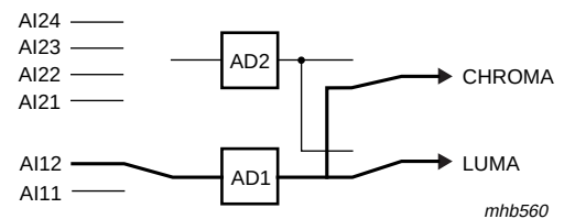
Fig 43. Mode 1 CVBS (automatic gain)
