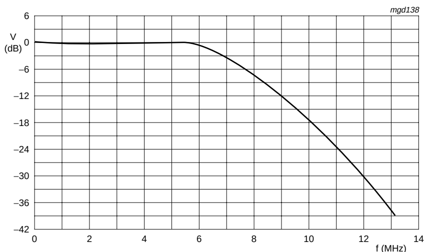
Fig 4. Anti-alias filter
