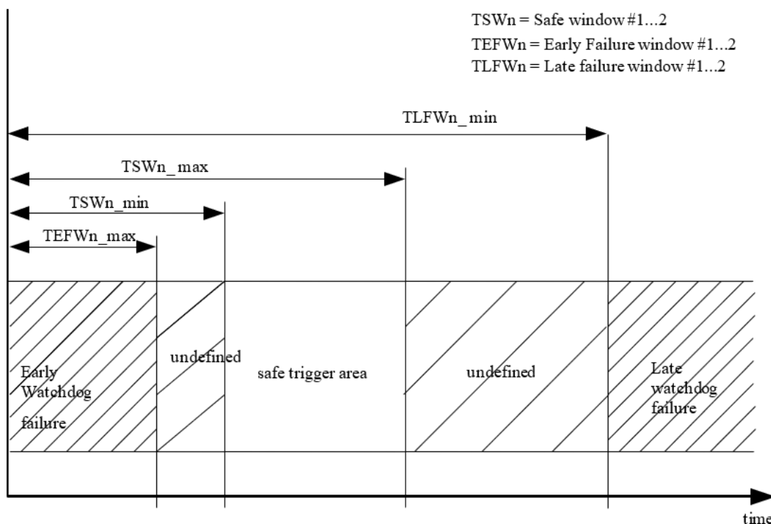
Figure 32. Watchdog early, late and safe windows
