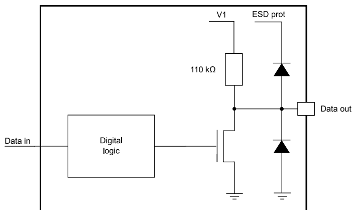
Figure 14. NRESET pin
