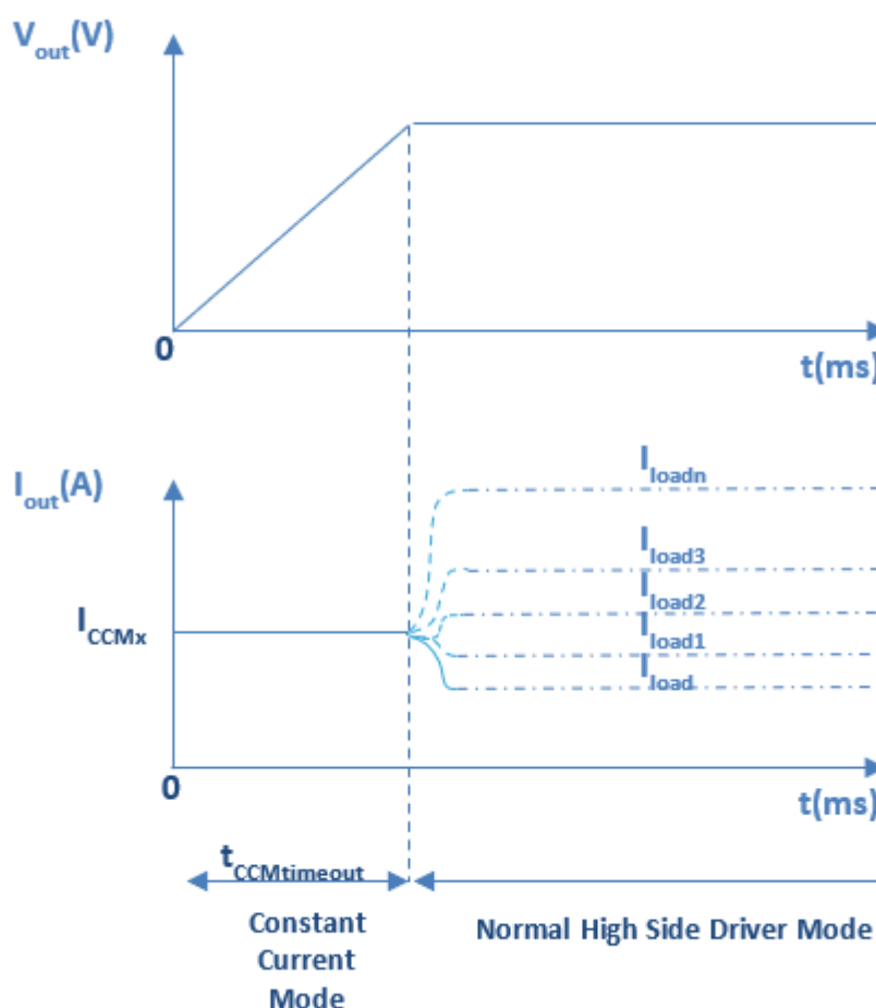
Figure 24. Constant current mode
