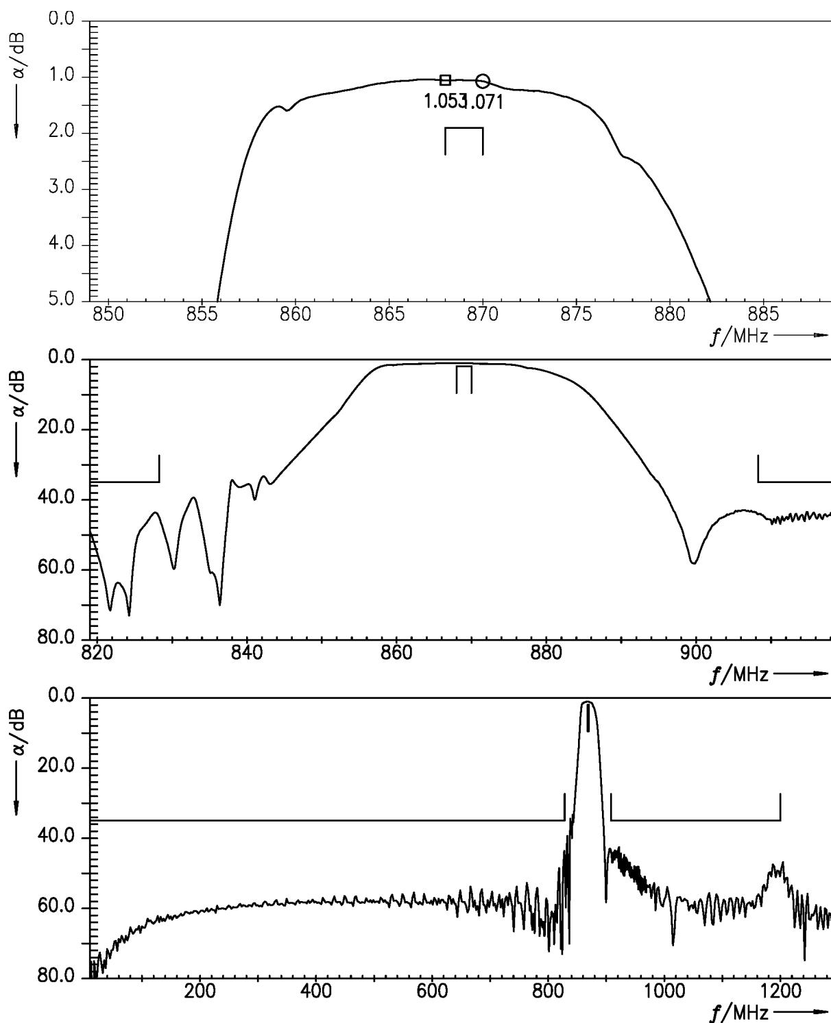
Figure 4: Attenuation .
