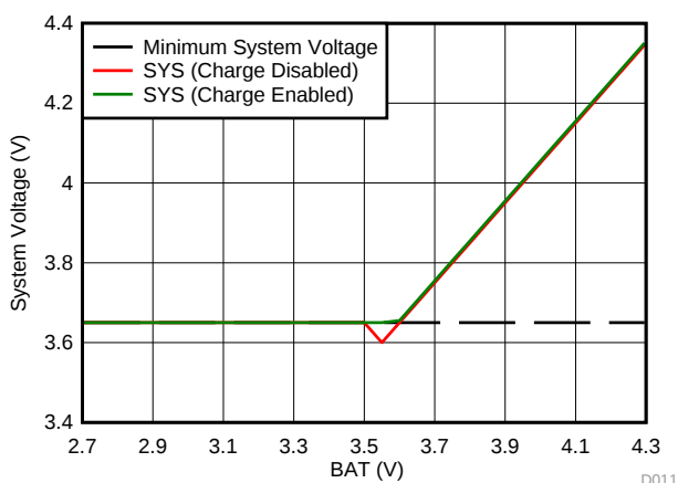
Figure 12. V(SYS) vs V(BAT)
