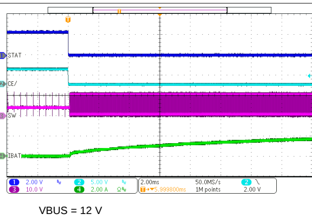
Figure 61. Charge Enable
