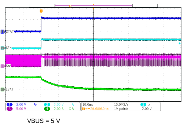
Figure 53. Charge Disable
