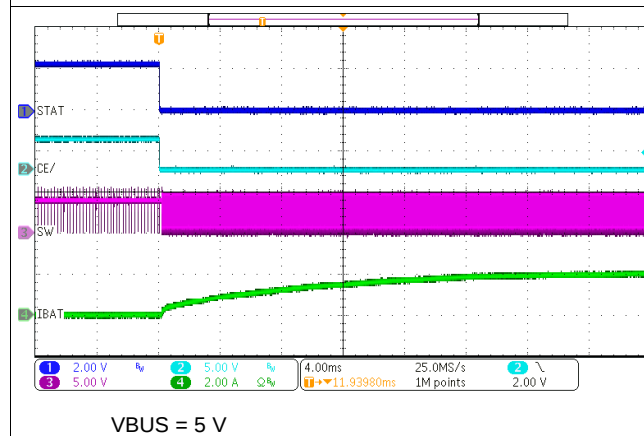
Figure 52. Charge Enable
