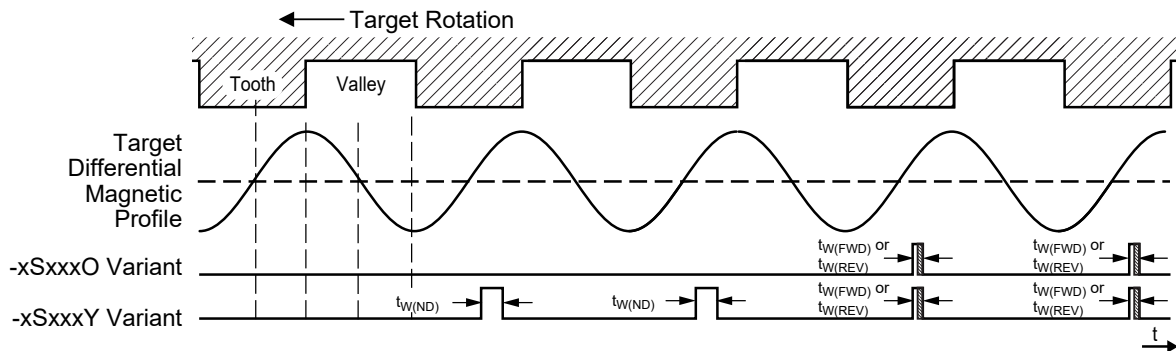
Figure 5: Output Options After Power-On
