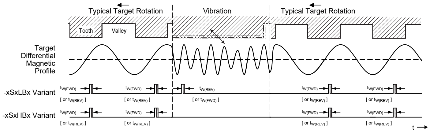
Figure 6: Output Functionality in the Presence of Running-Mode Target Vibration
