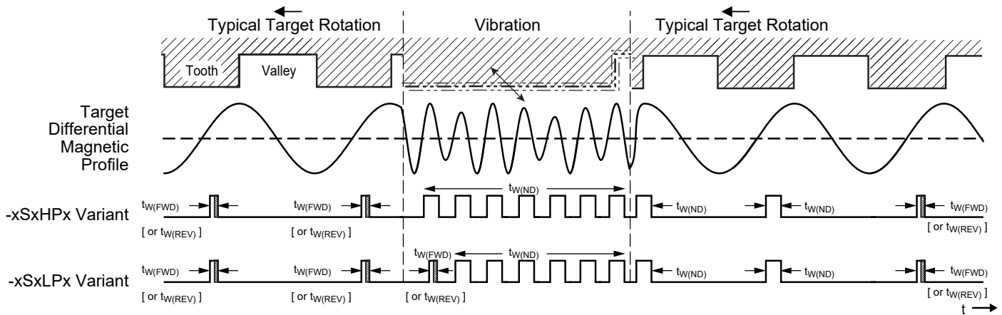
Figure 7: Output Functionality in the Presence of Running-Mode Target Vibration with Nondirectional Pulses
