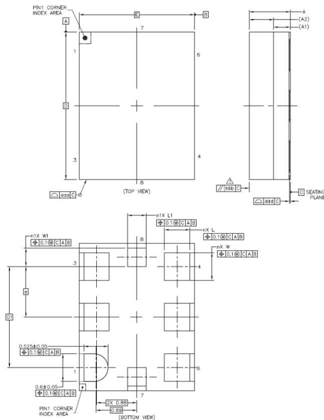
Figure 6.3. Si569 (2.5x3.2 mm) Outline Diagram
