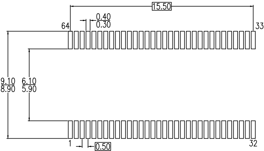
RECOMMENDED LAND PATTERN DIMENSIONS
