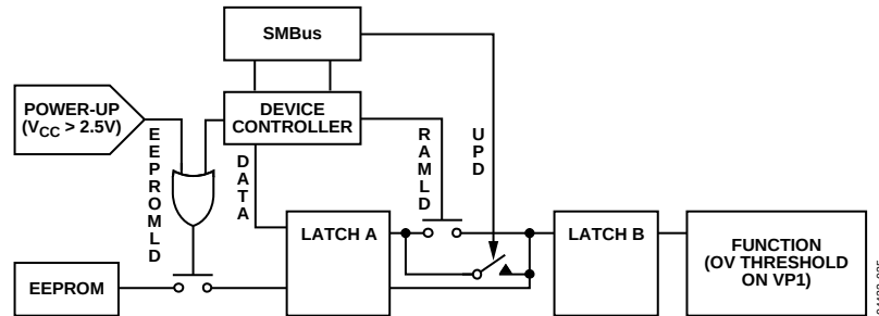
Figure 38. Configuration Update Flow Diagram
