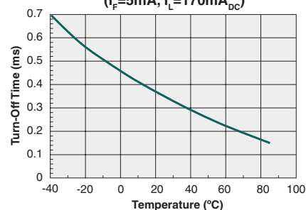
Typical Turn-Off Time vs. Temperature ( I_F=5\text{mA} , I_L=170\text{mA}_{DC} )
