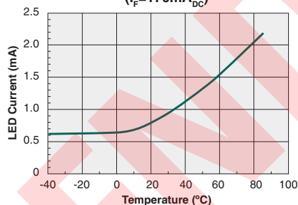
Typical I_F for Switch Dropout vs. Temperature ( I_F=170\text{mA}_{DC} )
