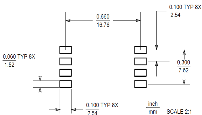
Figure 5. SOP Footprint
