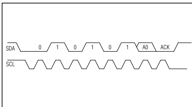
Figure 9. Slave Address
