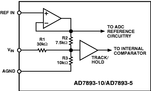
Figure 2. AD7893-10/AD7893-3/AD7893-5 Analog Input Structure
