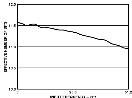
Figure 13. Effective Number of Bits vs. Frequency
