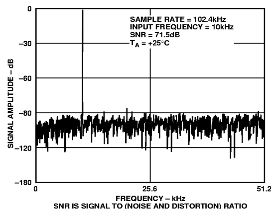
Figure 12. AD7893 FFT Plot
