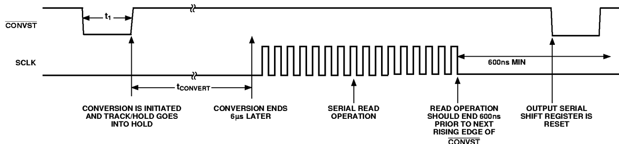
Figure 3. Timing Sequence for Optimum Performance from the AD7893
