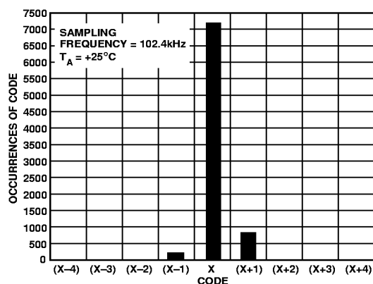
Figure 11. Histogram of 8192 Conversions with Read During Conversion
