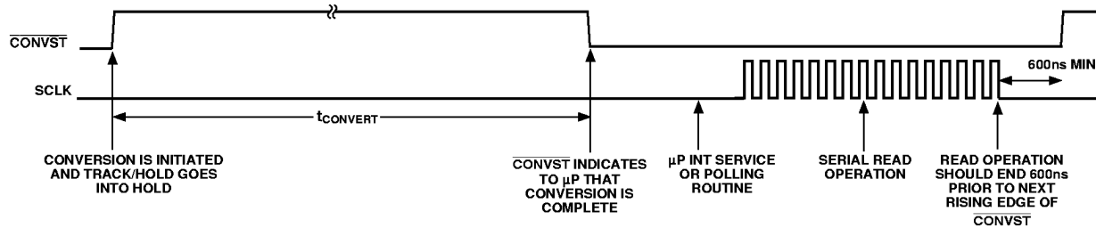
Figure 4. \overline{\text{CONVST}} Used as Status Signal
