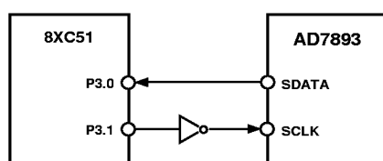
Figure 6. AD7893 to 8XC51 Interface
