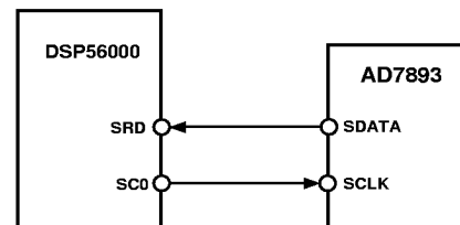
Figure 9. AD7893 to DSP56000 Interface
