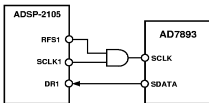
Figure 8. AD7893 to ADSP-2105 Interface
