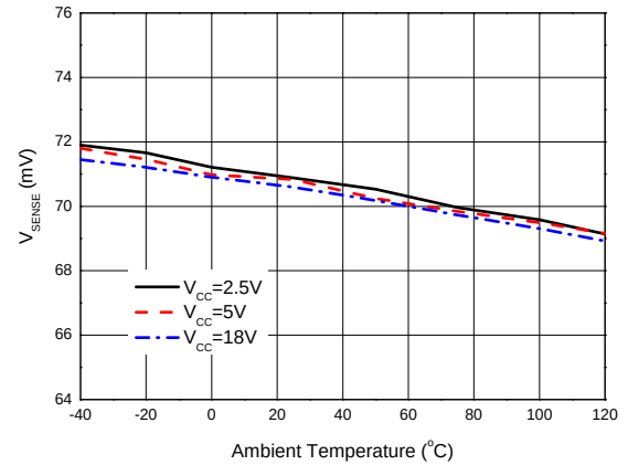
AP4306A V_{SENSE} vs. Ambient Temperature
