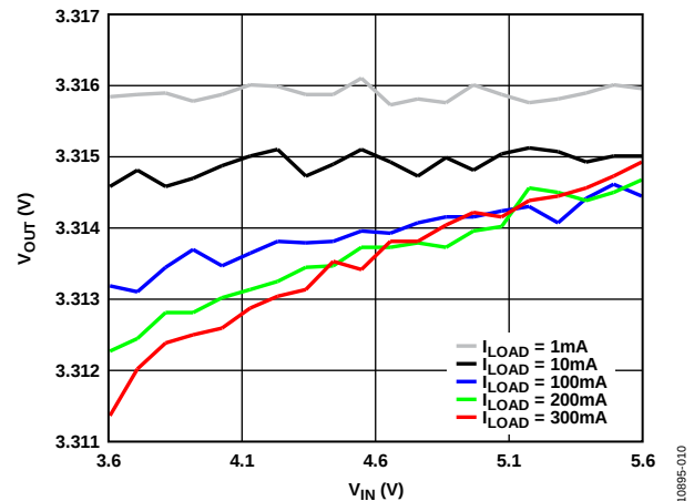
Figure 13. V_{OUT} vs. V_{IN} LDO Line Regulation for an Output of 3.3 V
