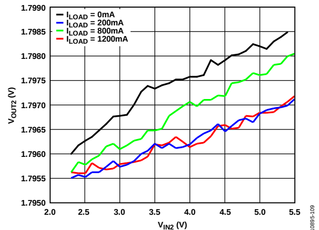
Figure 10. Buck Regulator Line Regulation, V_{OUT2} = 1.8\text{ V}
