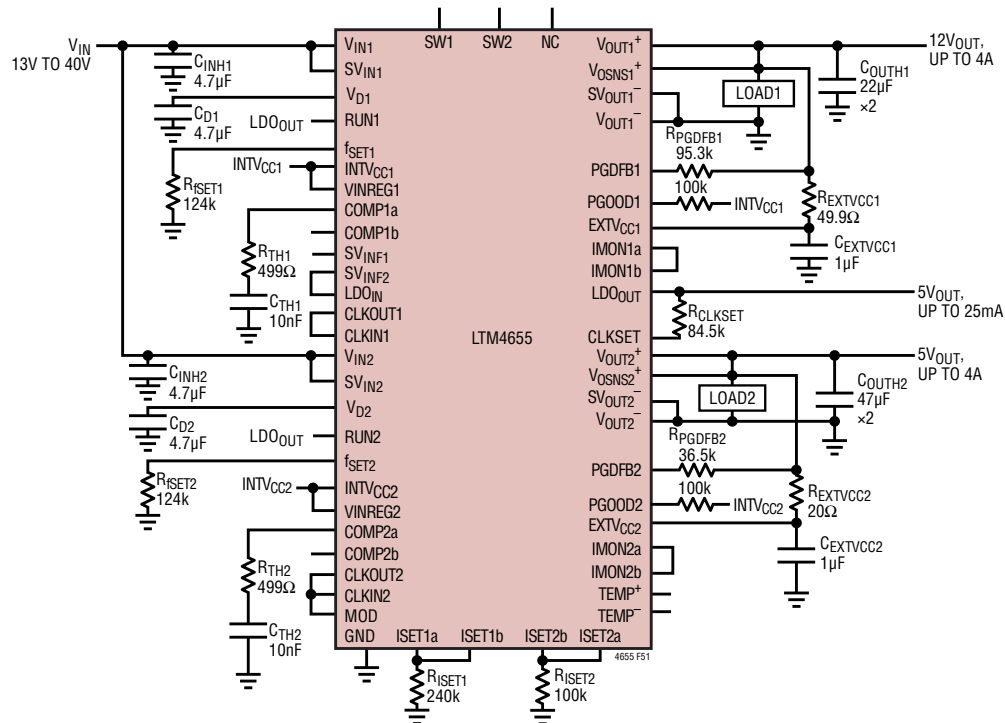
Figure 51. Dual 4A, 12V and 5V Output DC/DC \mu\text{Module} Regulator
