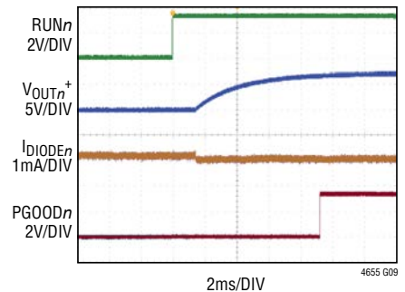
FIGURE 51 CIRCUIT, 36V_{IN} , C_{INHn} = C_{Dn} = 4.7\mu\text{F} , C_{OUTn} = 2 \times 22\mu\text{F} , R_{ISETn} = 124k , R_{ISETn} = 240k\Omega , R_{PGDFBn} = 95.3k\Omega , C_{THn} = 10nF , R_{THn} = 562\Omega , R_{EXTVCCn} = 49.9\Omega , C_{EXTVCCn} = 1\mu\text{F} , V_{OUTn}^+ PRE-BIASED TO 5V THROUGH 1N4148 DIODE
