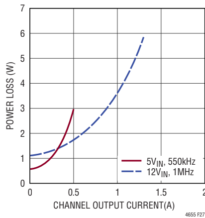
Figure 27. -24V OUT Power Loss Curve
