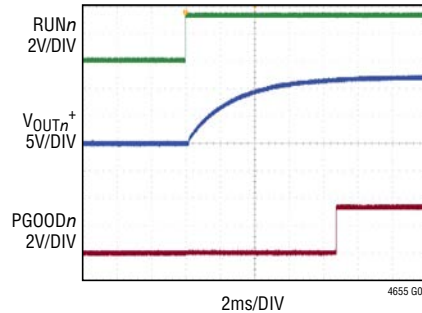
FIGURE 51 CIRCUIT, 36V_{IN} , C_{INHn} = C_{Dn} = 4.7\mu\text{F} , C_{OUTn} = 2 \times 22\mu\text{F} , R_{ISETn} = 124k , R_{ISETn} = 240k\Omega , R_{PGDFBn} = 95.3k\Omega , C_{THn} = 10nF , R_{THn} = 562\Omega , R_{EXTVCCn} = 49.9\Omega , C_{EXTVCCn} = 1\mu\text{F} , 3\Omega RESISTIVE LOAD
