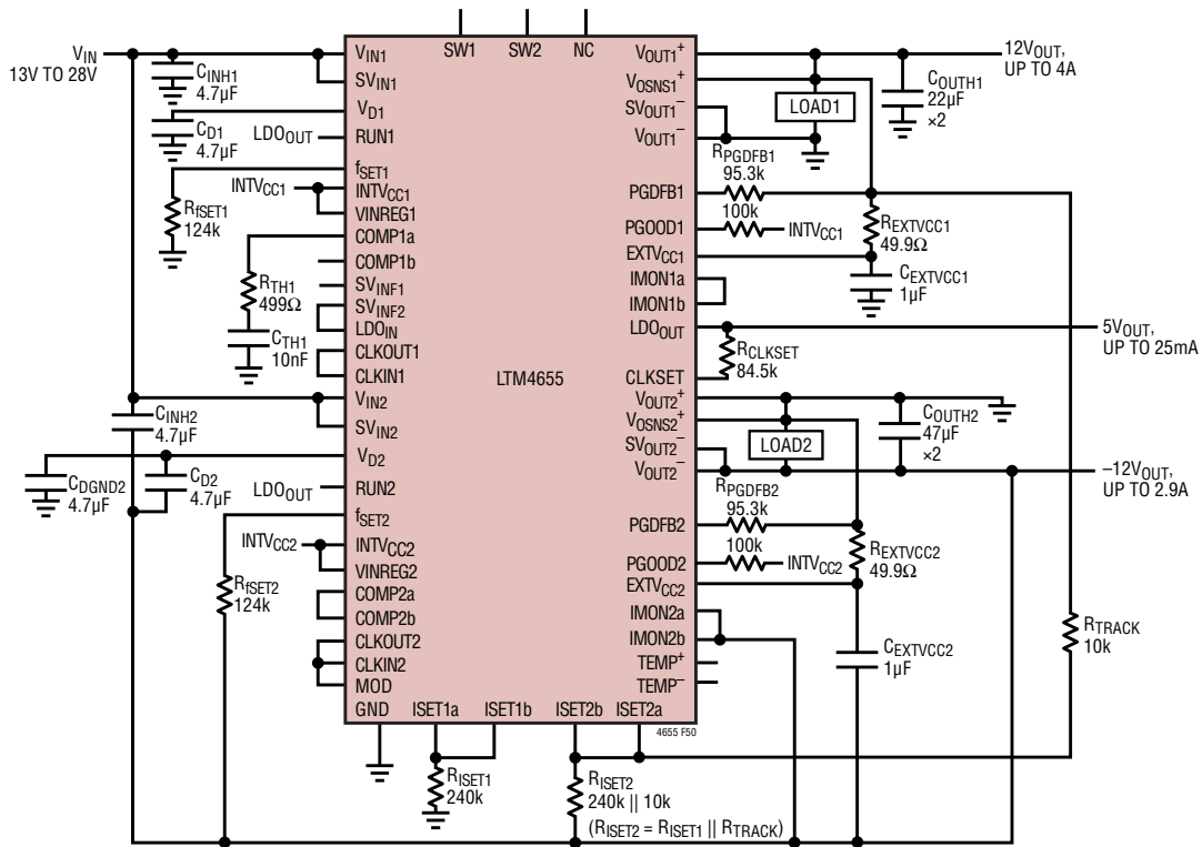
Figure 50. Concurrent \pm 12\text{V} Output DC/DC \mu\text{Module} Regulator
