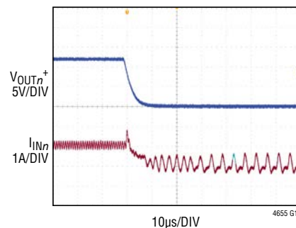
FIGURE 51 CIRCUIT, 36V_{IN} , C_{INHn} = C_{Dn} = 4.7\mu\text{F} , C_{OUTn} = 2 \times 22\mu\text{F} , R_{ISETn} = 124k , R_{ISETn} = 240k\Omega , R_{PGDFBn} = 95.3k\Omega , C_{THn} = 10nF , R_{THn} = 562\Omega , R_{EXTVCCn} = 49.9\Omega , C_{EXTVCCn} = 1\mu\text{F} , 4\Omega RESISTIVE LOAD PRIOR TO APPLICATION OF OUTPUT SHORT-CIRCUIT
