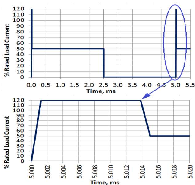
Figure 16. AC-DC Load Profile
