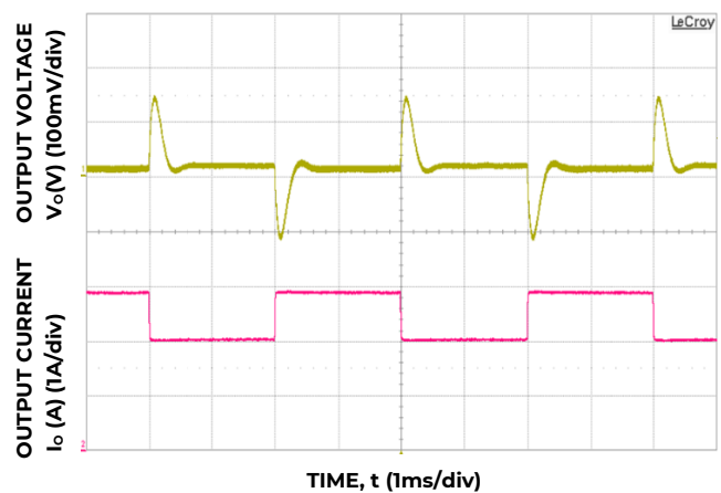
Figure 6. Dynamic Load Change Transient Response from 50% to 75% to 50% of Full Load at Room Temperature and 48V in ; 0.1A/μS, C_{o,ext} = 220\mu F .
