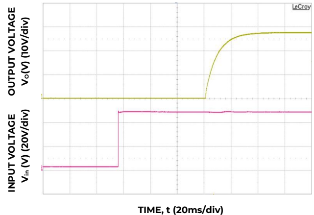
Figure 5. Typical Start-Up from V IN , on/off enabled prior to V IN step; C_{o,ext} = 220\mu F .
