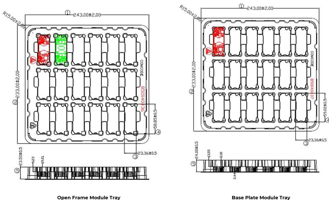
Figure 25. ERCW003A6R Packaging Tray
