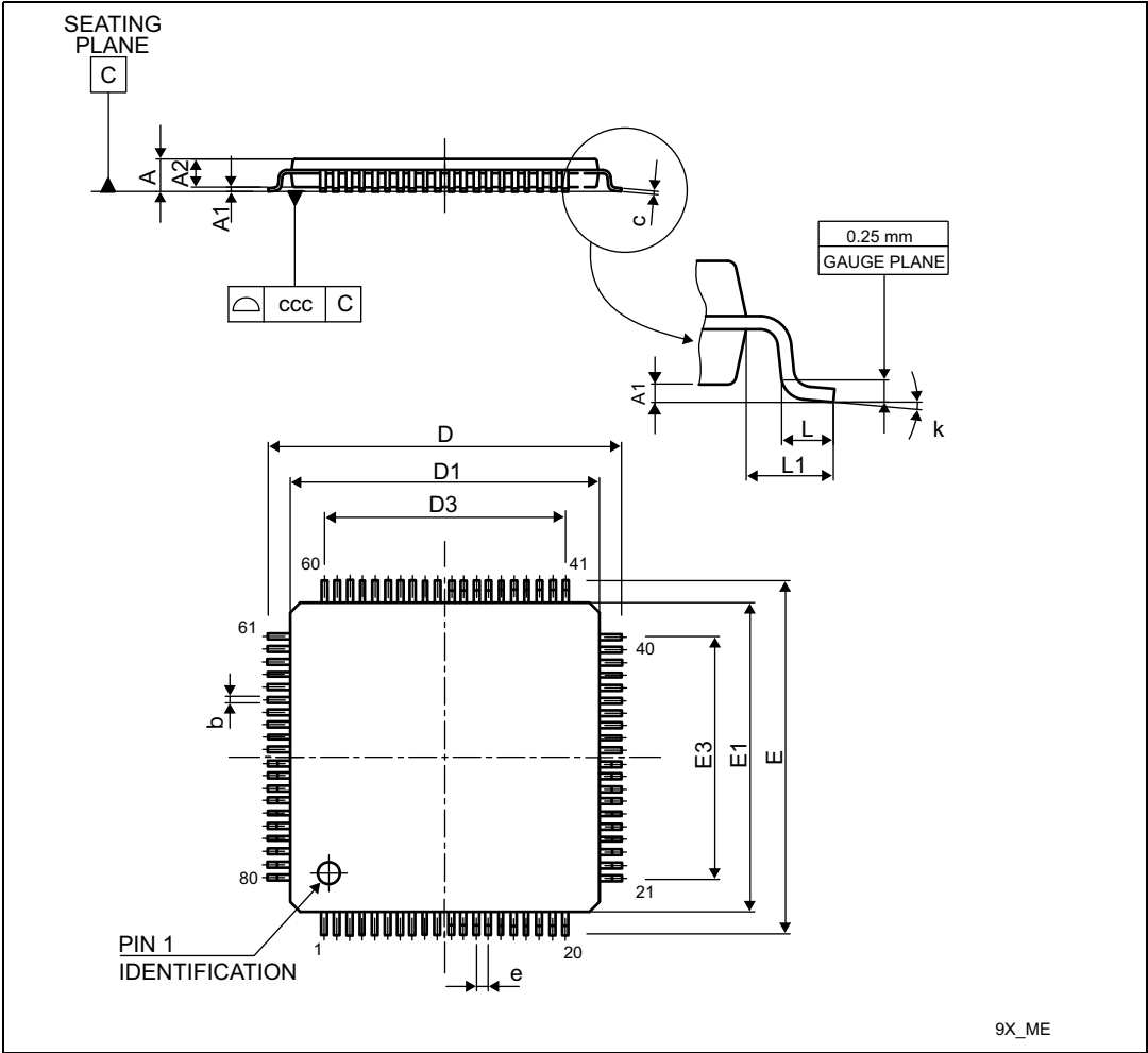
Figure 61. LQFP80 - Outline
