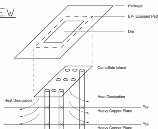
PCB Thermal Consideration for 32-Pin MFL® Package (Always solder, or equivalent, the exposed pad to the PCB)
