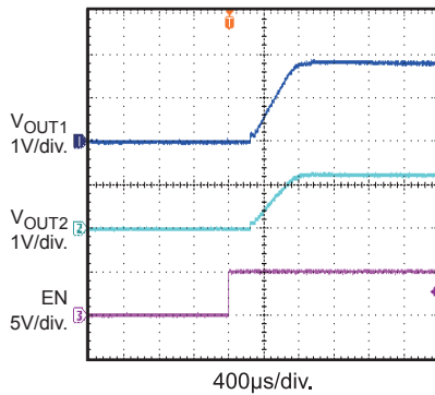
EN On without Load IOUT1 = IOUT2 = 0A
