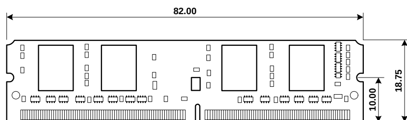
Figure: mechanical dimensions 1
