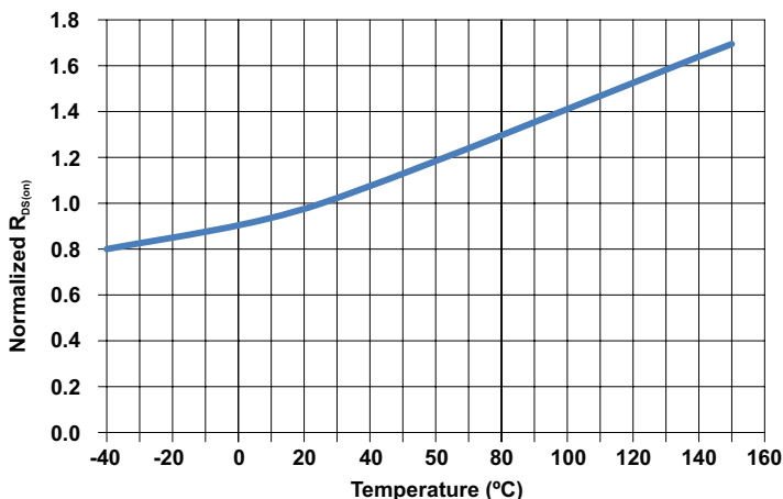
Figure 3: Typical MOSFET R_{DS(on)} versus Temperature
