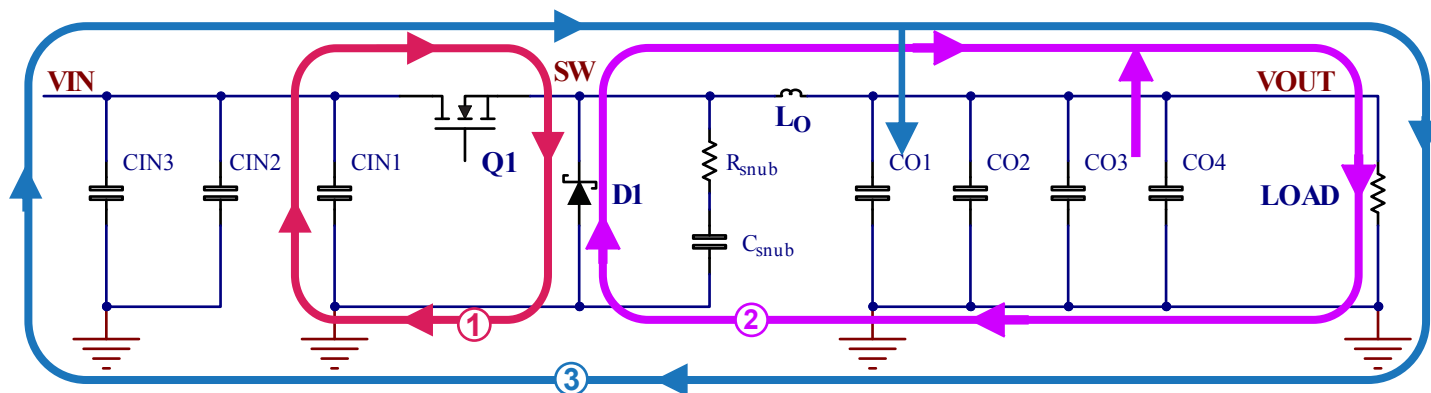
Figure 24: Typical Buck Converter with Critical Paths/Loops Shown
