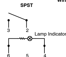
Wiring Diagram
