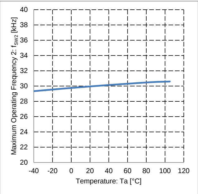
Figure 41. Maximum Operating Frequency 2 vs Temperature
