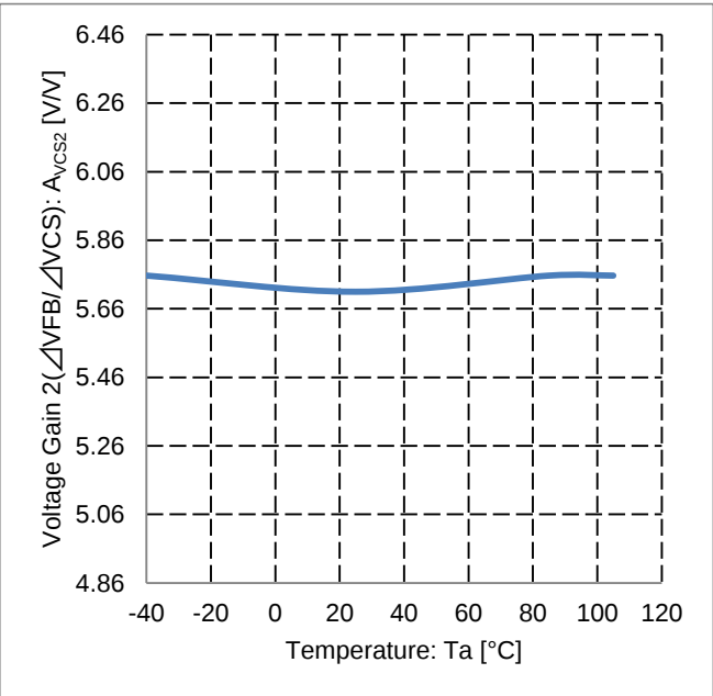
Figure 37. Voltage Gain 2 ( \Delta V_{FB}/\Delta V_{CS} ) vs Temperature
