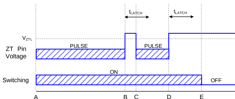
Figure 20. ZT OVP and Latch Mask Function
