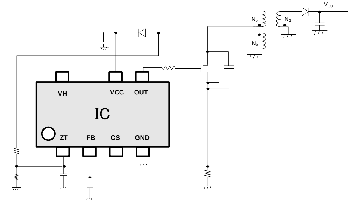
Figure 9. VCC OVP
