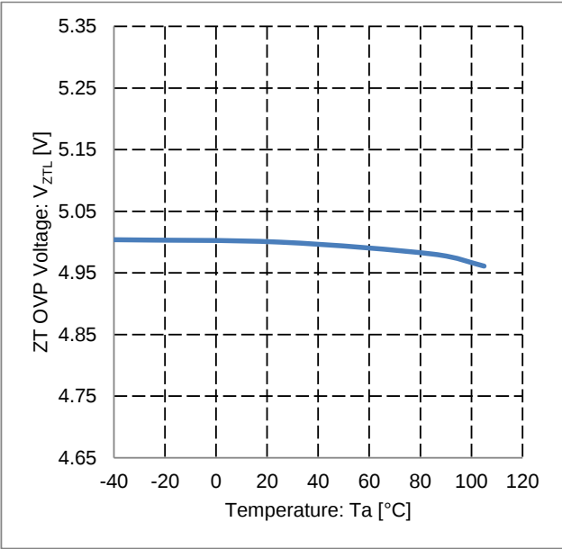
Figure 52. ZT OVP Voltage vs Temperature
