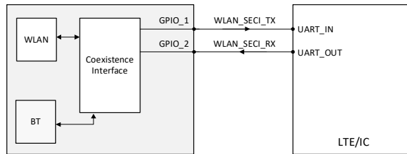
Figure 27. 2-Wire Coexistence Interface to an External IC
