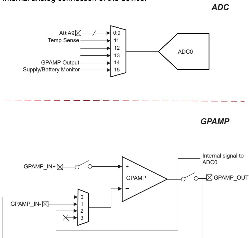
Figure 8-1. Analog Connections
