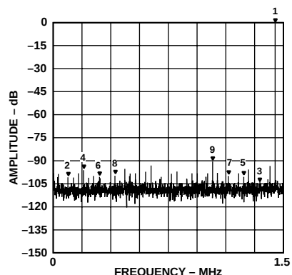
Figure 7. Typical FFT, f_{\text{IN}} = 1.50 \text{ MHz} (Input Span = 2 V, V_{\text{CM}} = 2.5 \text{ V} )
