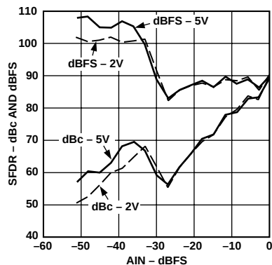
Figure 9. Single Tone SFDR ( f_{\text{IN}} = 1.5 \text{ MHz} , V_{\text{CM}} = 2.5 \text{ V} )
