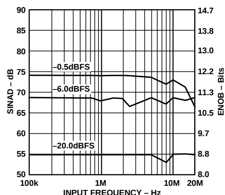
Figure 5. SINAD vs. Input Frequency (Input Span = 2 V, V_{\text{CM}} = 2.5 \text{ V} )
