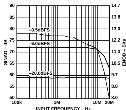
Figure 2. SINAD vs. Input Frequency (Input Span = 5 V, V_{\text{CM}} = 2.5 \text{ V} )
