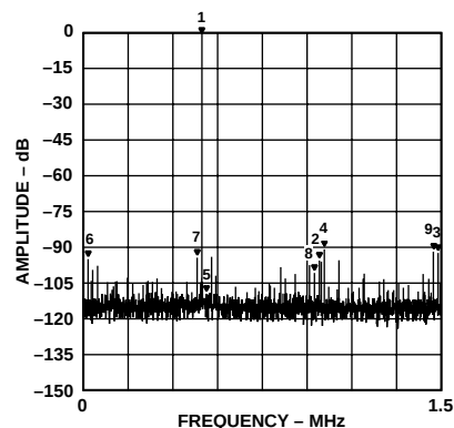
Figure 4. Typical FFT, f_{\text{IN}} = 500 \text{ kHz} (Input Span = 5 V, V_{\text{CM}} = 2.5 \text{ V} )
