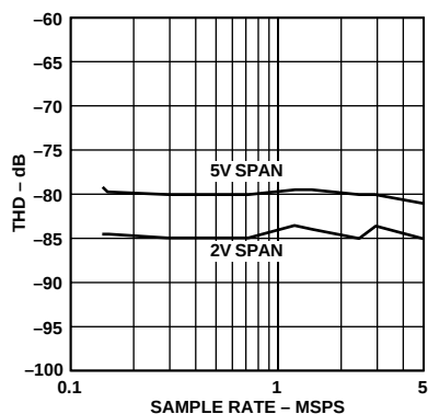
Figure 8. THD vs. Sample Rate ( f_{\text{IN}} = 1.5 \text{ MHz} , A_{\text{IN}} = -0.5 \text{ dBFS} , V_{\text{CM}} = 2.5 \text{ V} )
