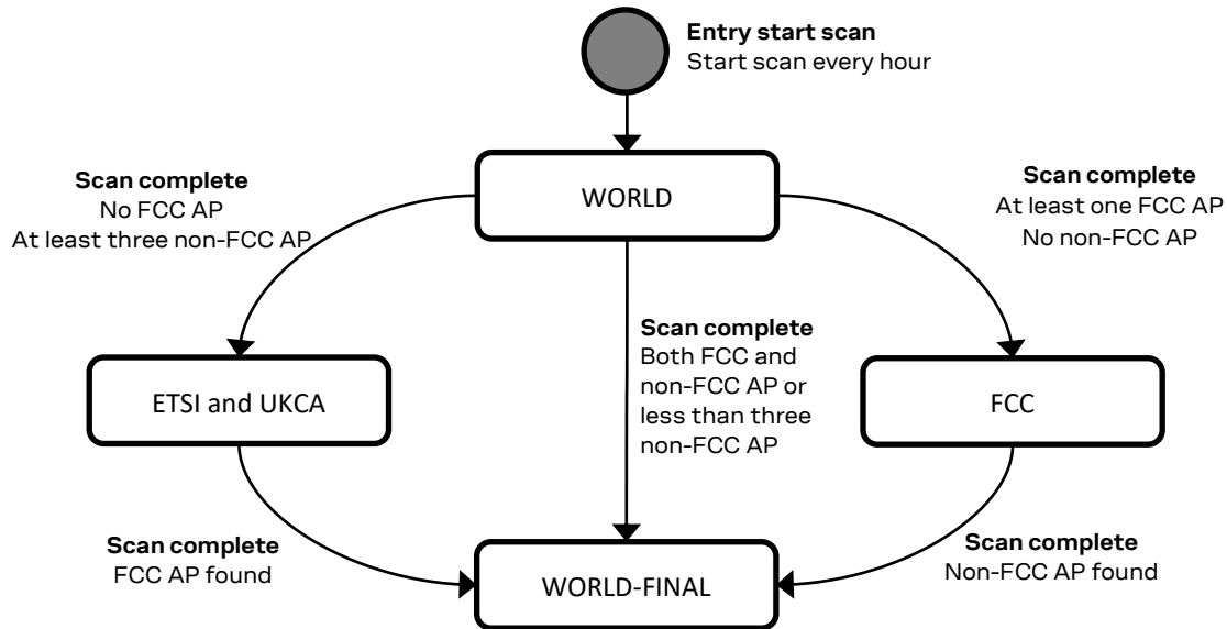
Figure 2: NINA-W15_DataSheet_UBX-18006647 IEEE 802.11d state transition diagram
