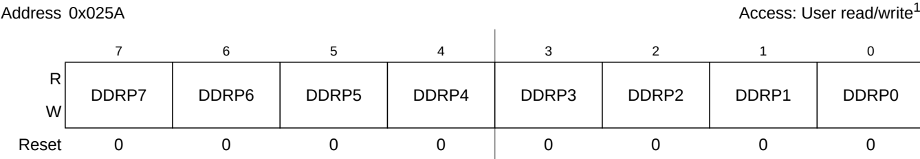
Figure 2-31. Port P Data Direction Register (DDRP)
