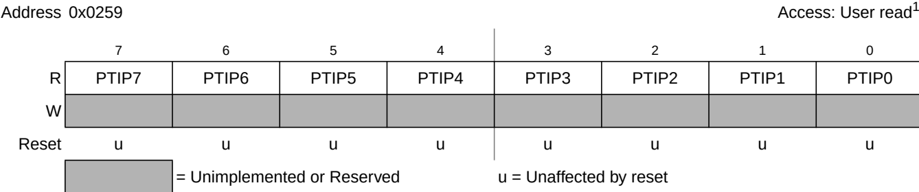
Figure 2-30. Port P Input Register (PTIP)
