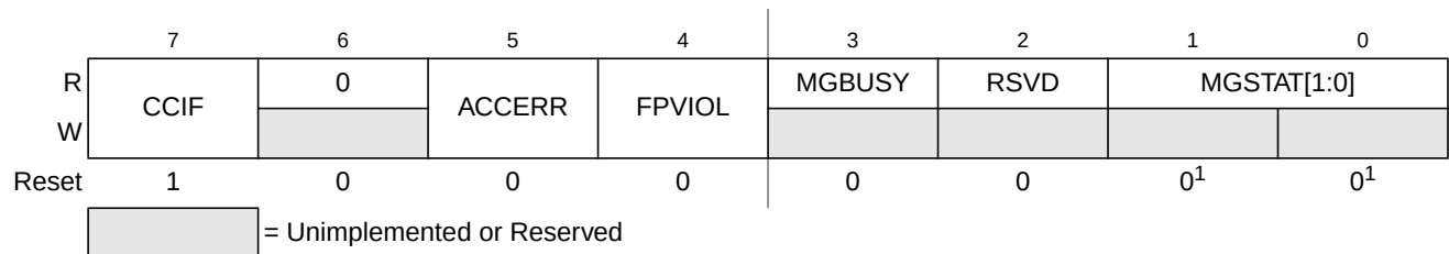
Figure 16-11. Flash Status Register (FSTAT)
