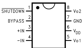
Figure 3. Mini Small Outline (VSSOP) Package – Top View See Package Number DGK
