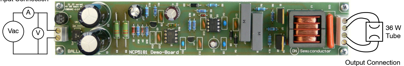
Figure 8. Ballast Connection
