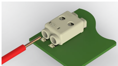
Insert solid conductors horizontal to printed circuit board to complete termination
