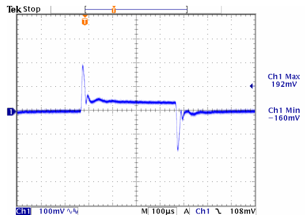
Figure 12. V_{in}=12V , V_{out}=5.0V
