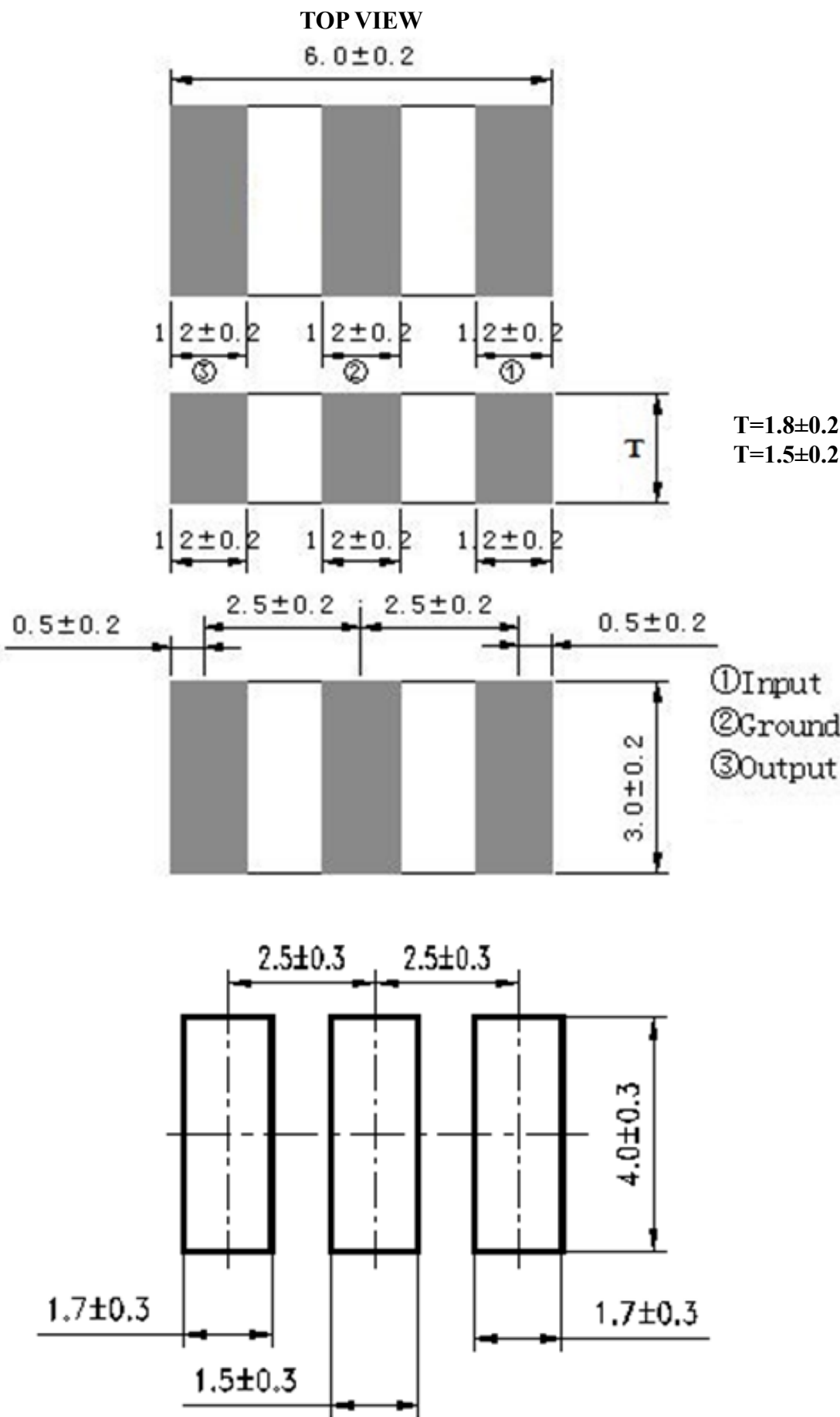
RECOMMENDED LANDING PATTERN (mm)
