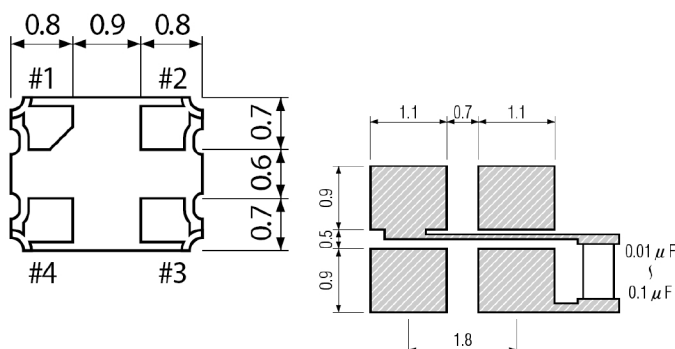
Figure 2) Suggested Land Pattern
