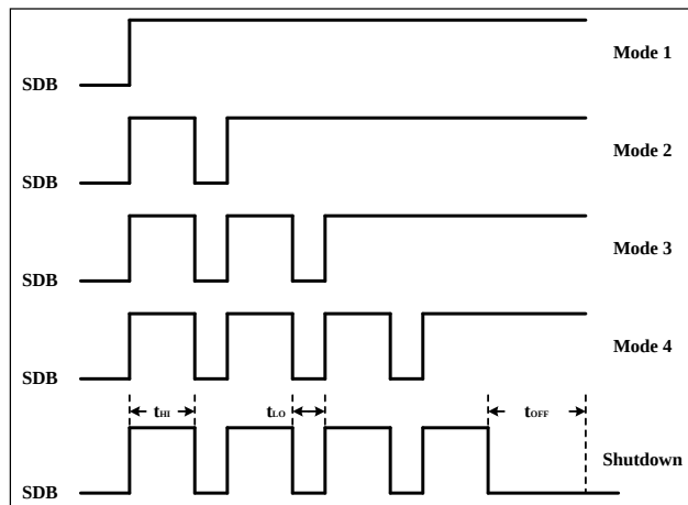
Figure 12 Operating Mode Control
