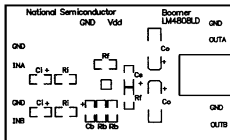
Figure 47. Recommended LD PC Board Layout: Top Silkscreen
