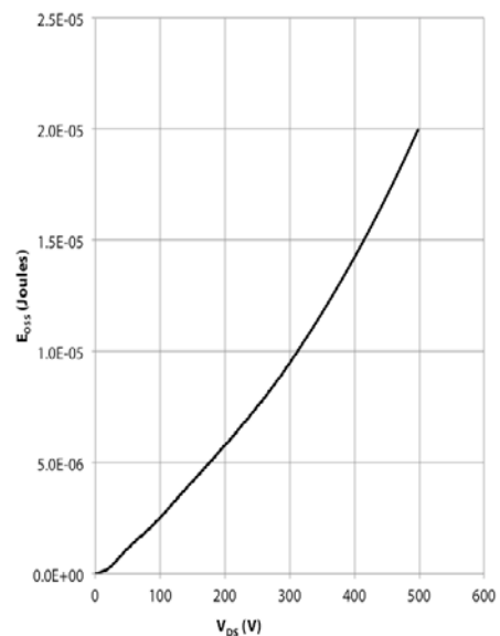
Figure 8: Typical C_{oss} Stored Energy
