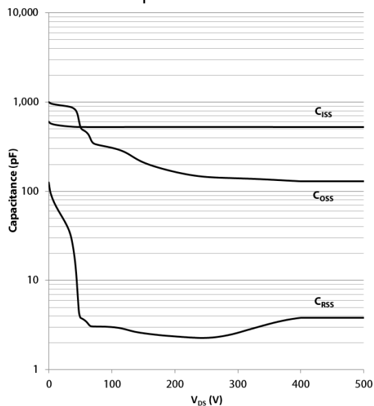
GS66516T Capacitance Characteristic
