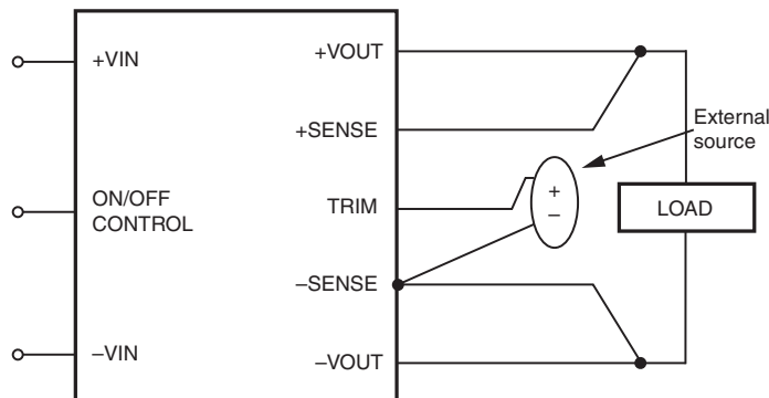
Figure 9. Trimming with an External Source
