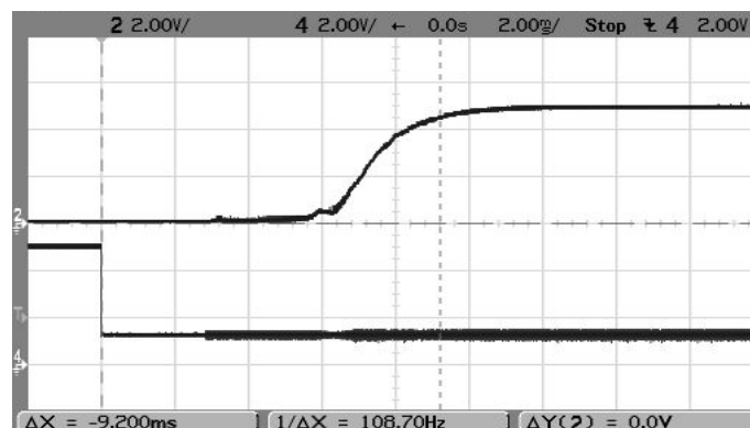
Enable Start-up (VIN=48V, Iout=12A, Load=1000uF, Ta=+25°C) Trace 2=Output, Trace 4= Enable.
