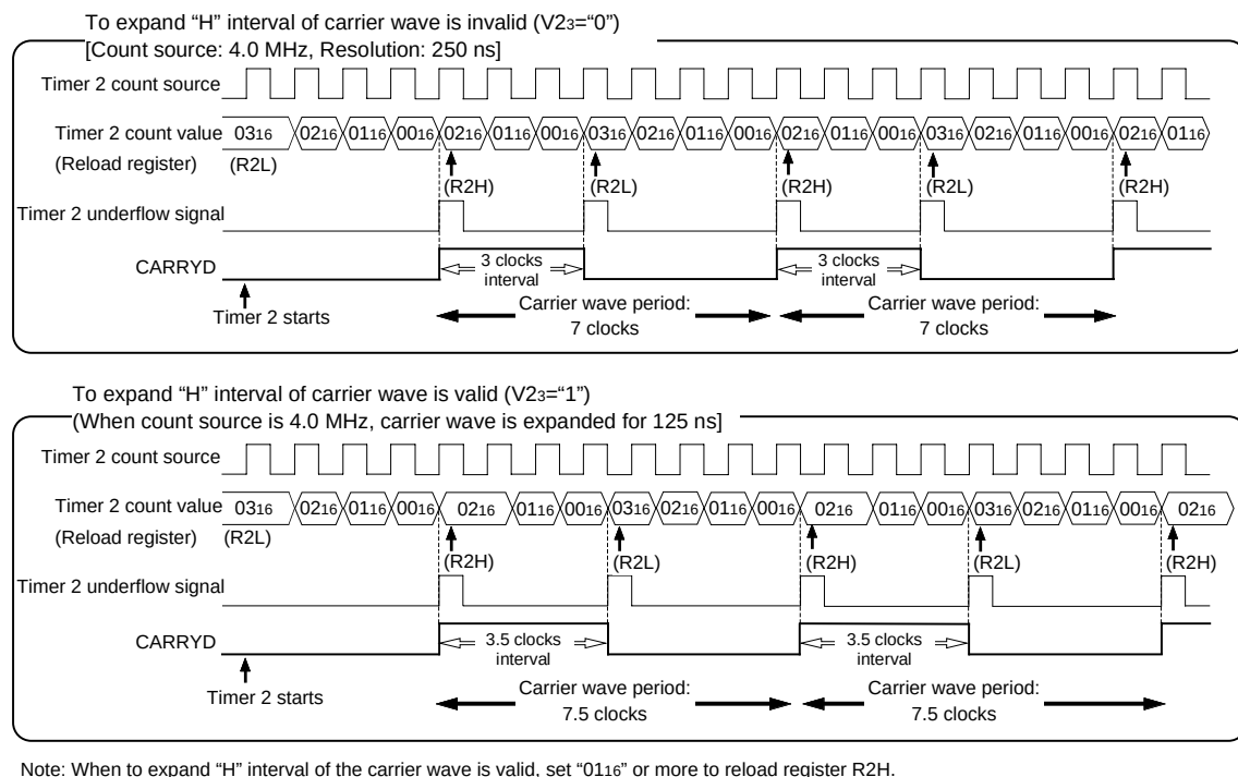
Fig. 16 Carrier wave generation example by timer 2
