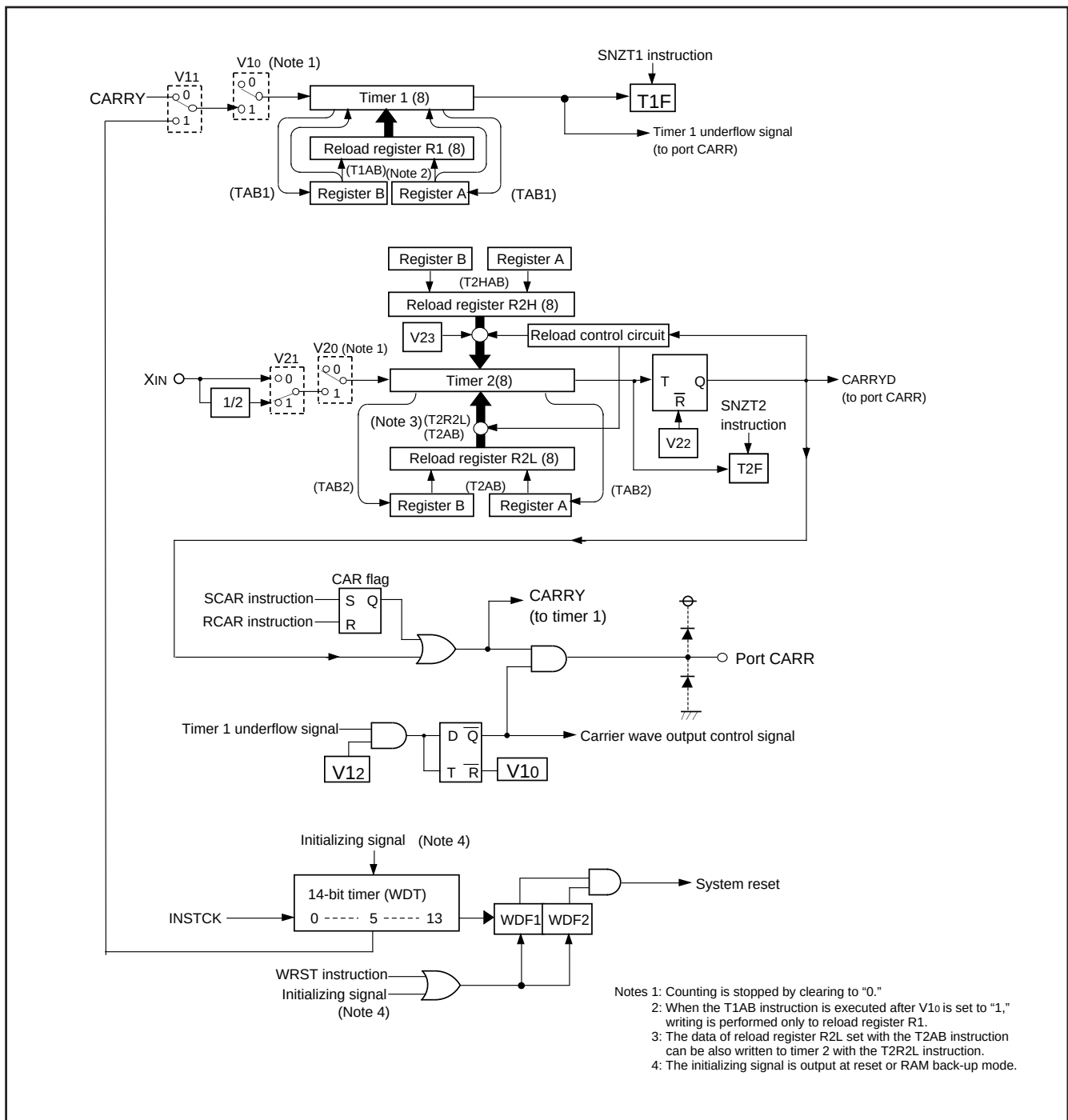
Fig. 13 Timers structure
