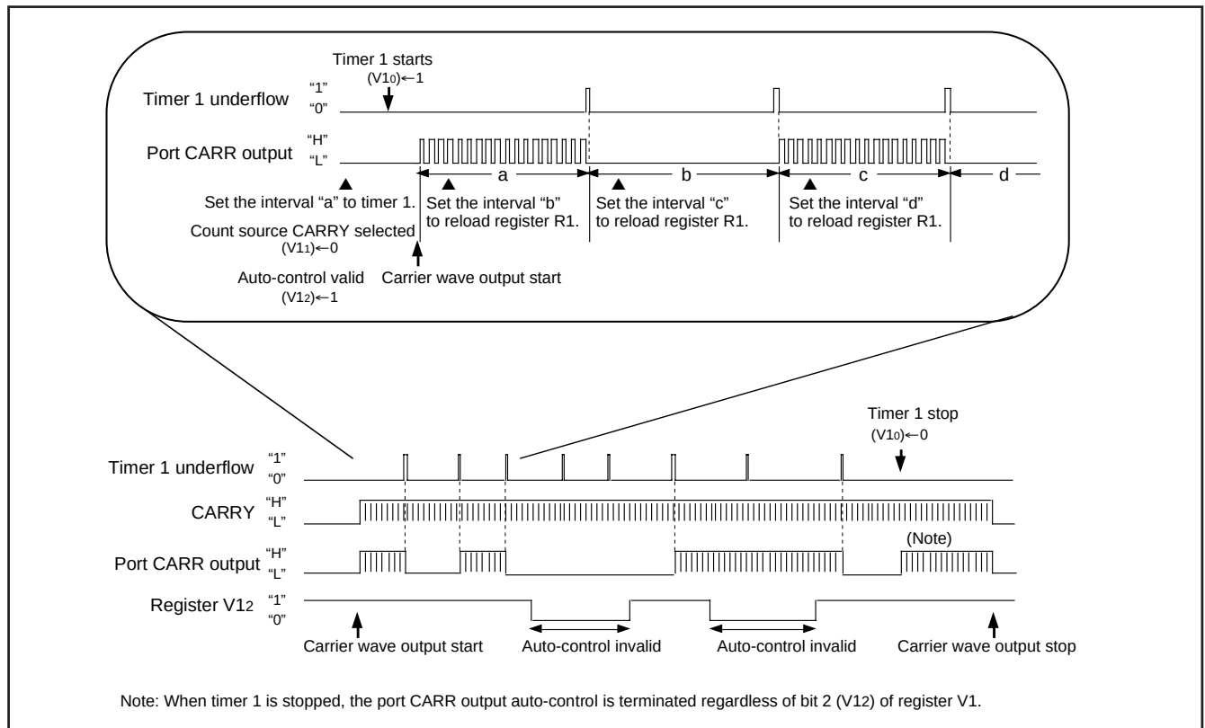
Fig. 15 Port CARR output control by timer 1
