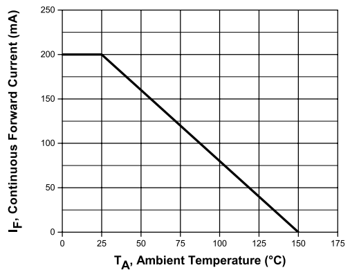
Current Derating
