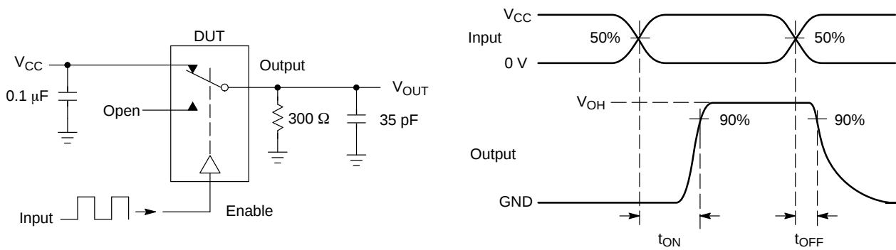
Figure 20. t_{\text{ON}}/t_{\text{OFF}}
