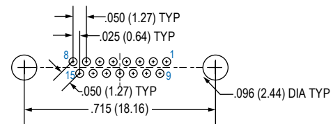
15 CONTACTS
