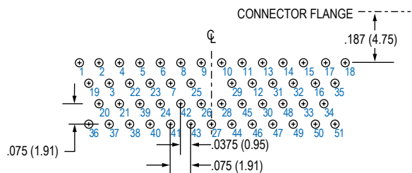
51 PIN
