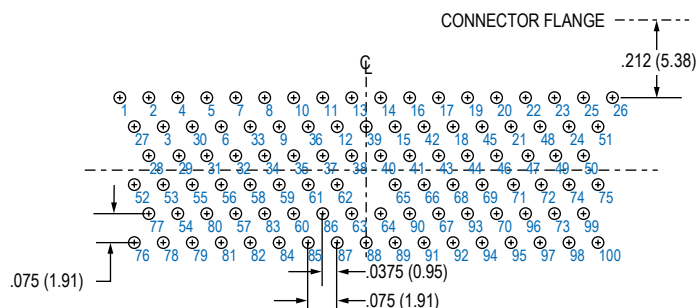
100 PIN
