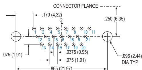
21 PIN
