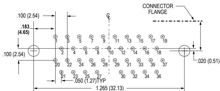
37 CONTACTS
