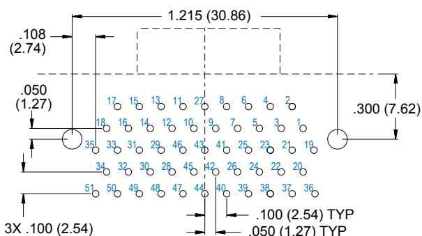
51 Socket
