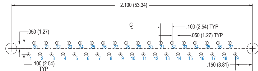
37 SOCKET M83513/25-F
