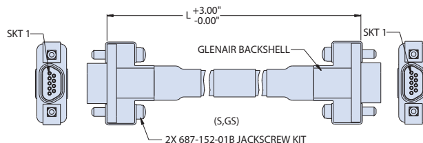
BACK TO BACK WIRING CABLE ASSY TYPE -AL ECSS-E-ST-50-12C REV 1, FIGURE 5-5
