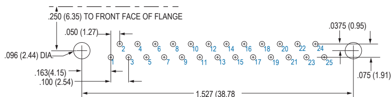
25 SOCKET
