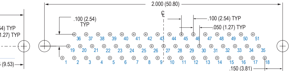
51 SOCKET M83513/26-G
