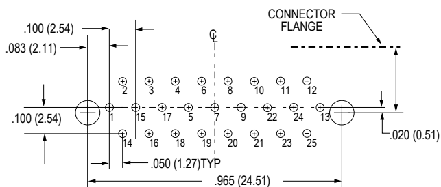
25 CONTACTS
