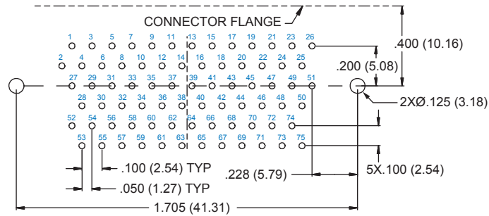
75 PIN
