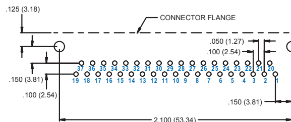
37 PIN M83513/16-F
