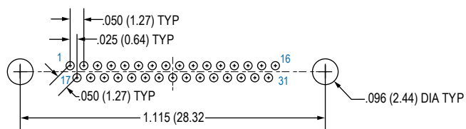
31 CONTACTS
