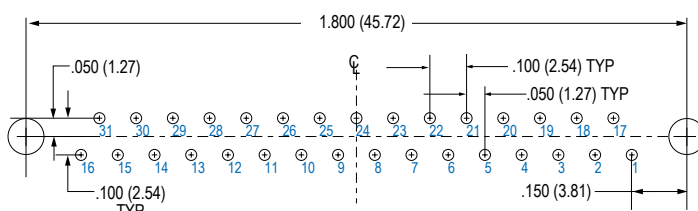
31 PIN
