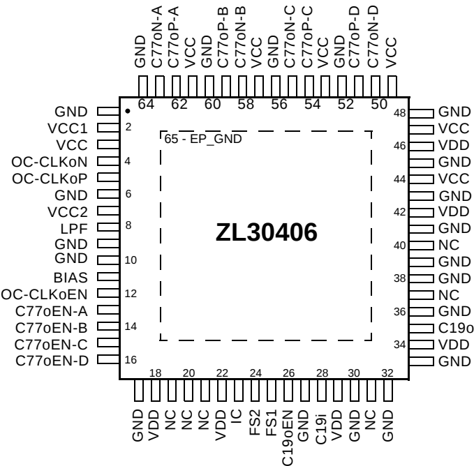
Figure 2 - TQFP 64 pin (Top View)
