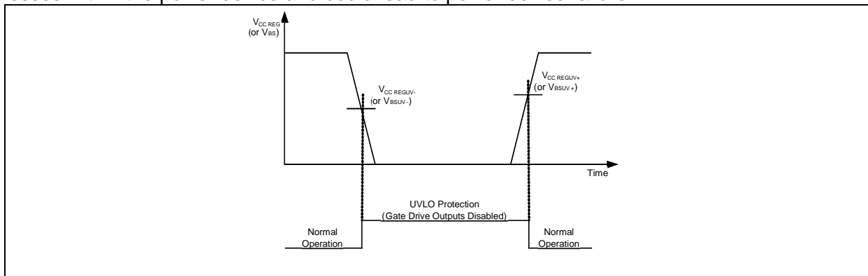
Figure 10 UVLO protection
