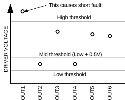
Figure 22. Short Fault
