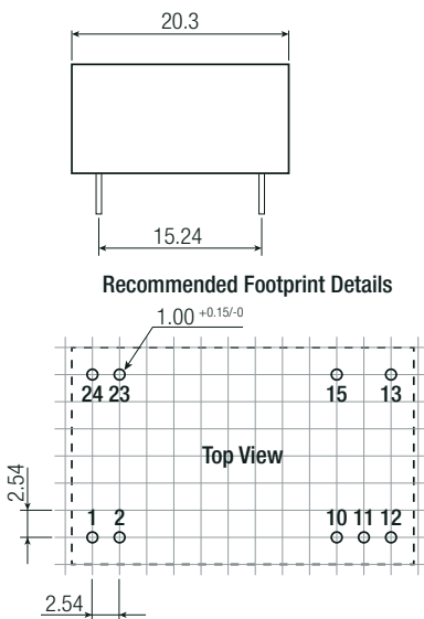
„C“ Pinning information (/H2, /H4, /H6)
